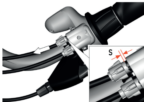
Image 39: Checking cable slack
